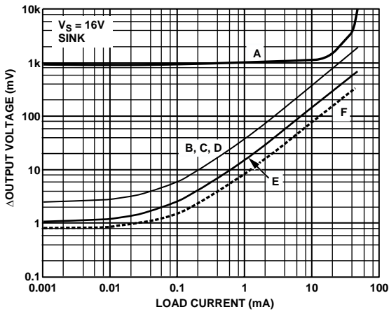
Figure 8. Output Sink Voltage vs. Load Current, All Channels
