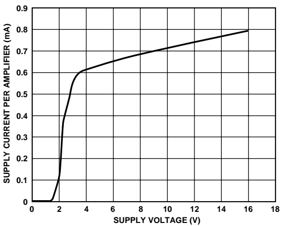
Figure 10. Supply Current vs. Supply Voltage
